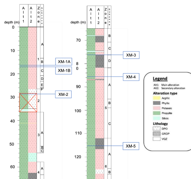
Figure 2 Column of the first 130 m of XM011. The drill core is divided in zones according to the observed changes in lithology/alteration (represented by numbers: 1-6) and subzones according differences of estimated total sulphide content and K-alteration (represented by letters: A-F).
