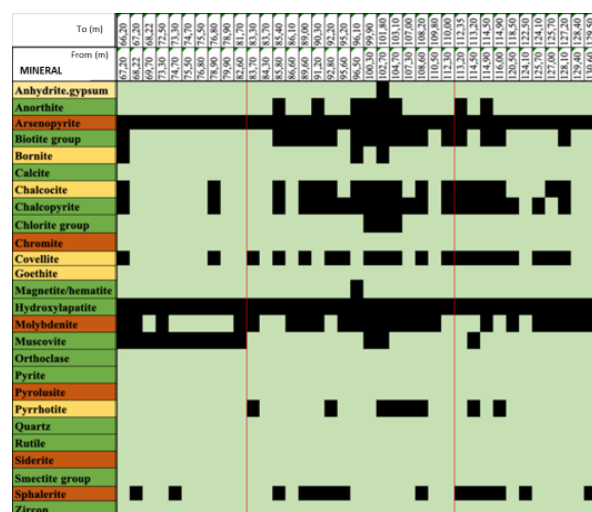
Figure 3 Refined list of minerals for the segment 66,20-130,60 m of XM001 after integrating all mineralogical/geochemical methods. The mineral names highlighted in green indicates direct observation and/or high probability of occurrence, whereas yellow represents less probability of occurrence. Those minerals listed in red were not discarded, but their probability of occurrence in the sample is low.
